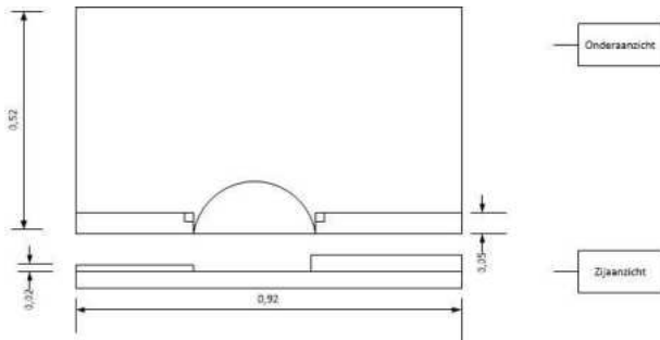
Fig. 10 Drawing of attachment
